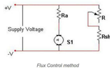
Flux Control method
