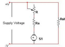
Armature Control method
