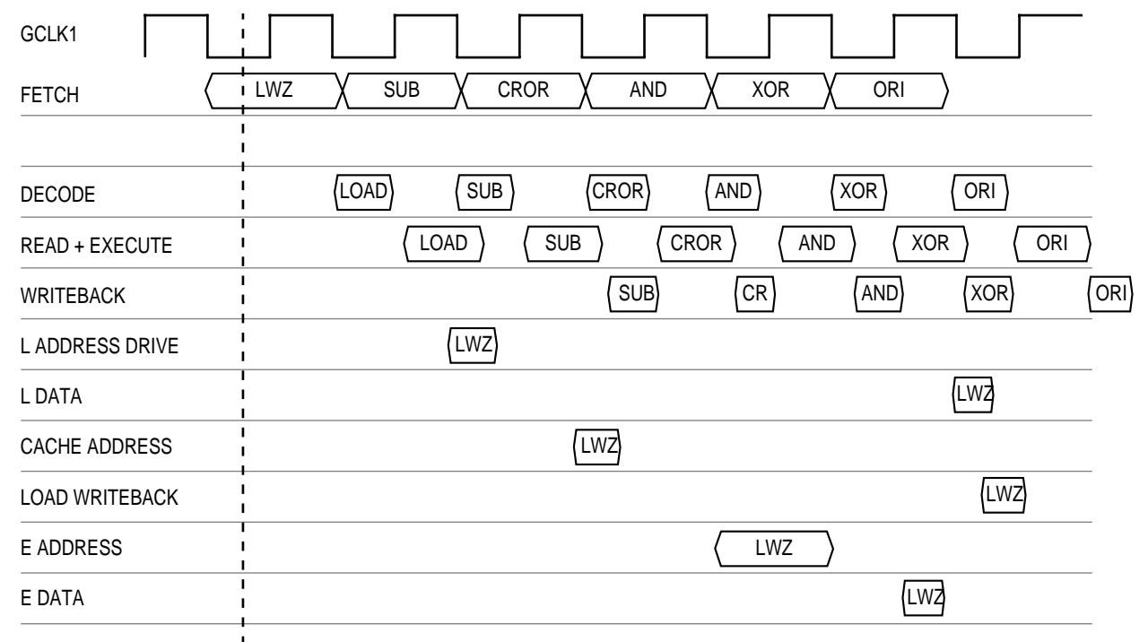
Figure 8-4. Example of a Private Writeback Bus Load
