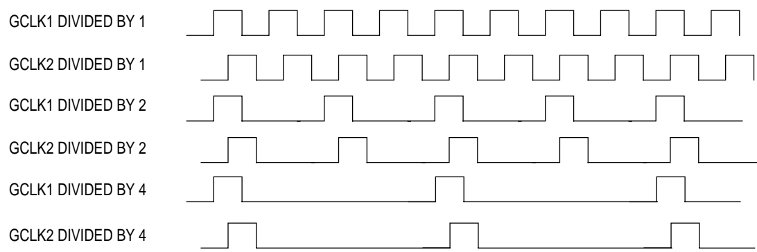
Figure 5-8. Divided System Clocks Timing Diagram
