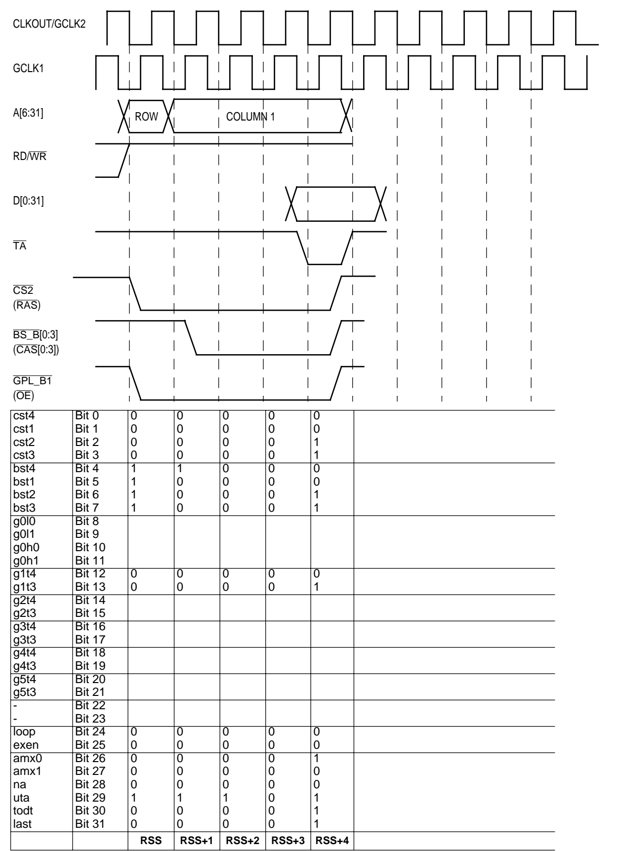
Figure 15-52. EDO DRAM Single Beat Read Access
