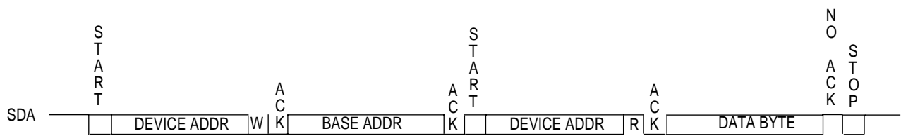
Figure 16-128. Byte Read from Device with Internal Addresses
