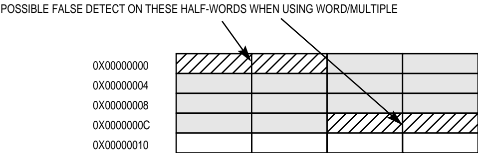
Figure 20-2. Example 2 False Detect on Watchpoint/Breakpoint
