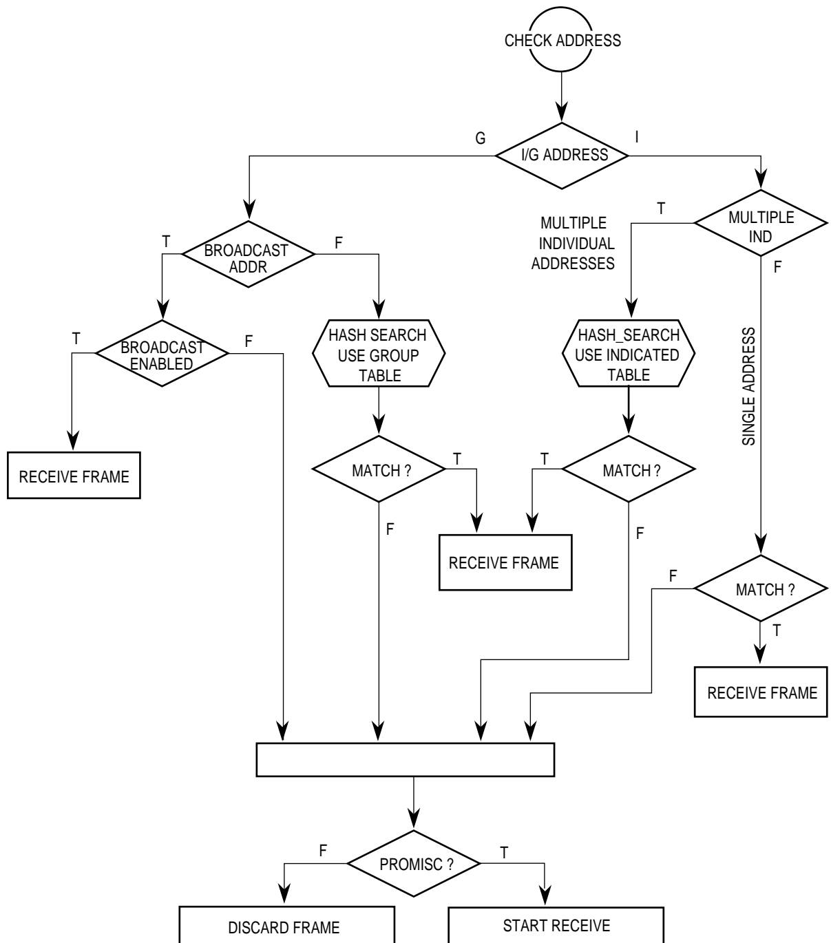
Figure 16-90. Reception Flowchart
