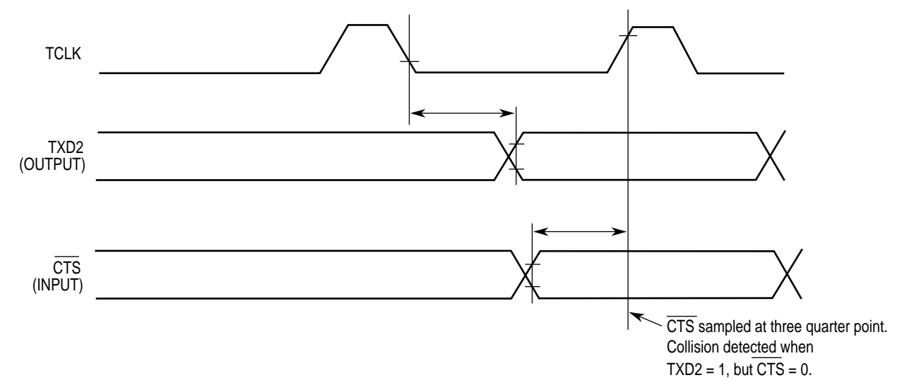
Figure 16-83. Example of a Nonsymmetrical Duty Cycle
