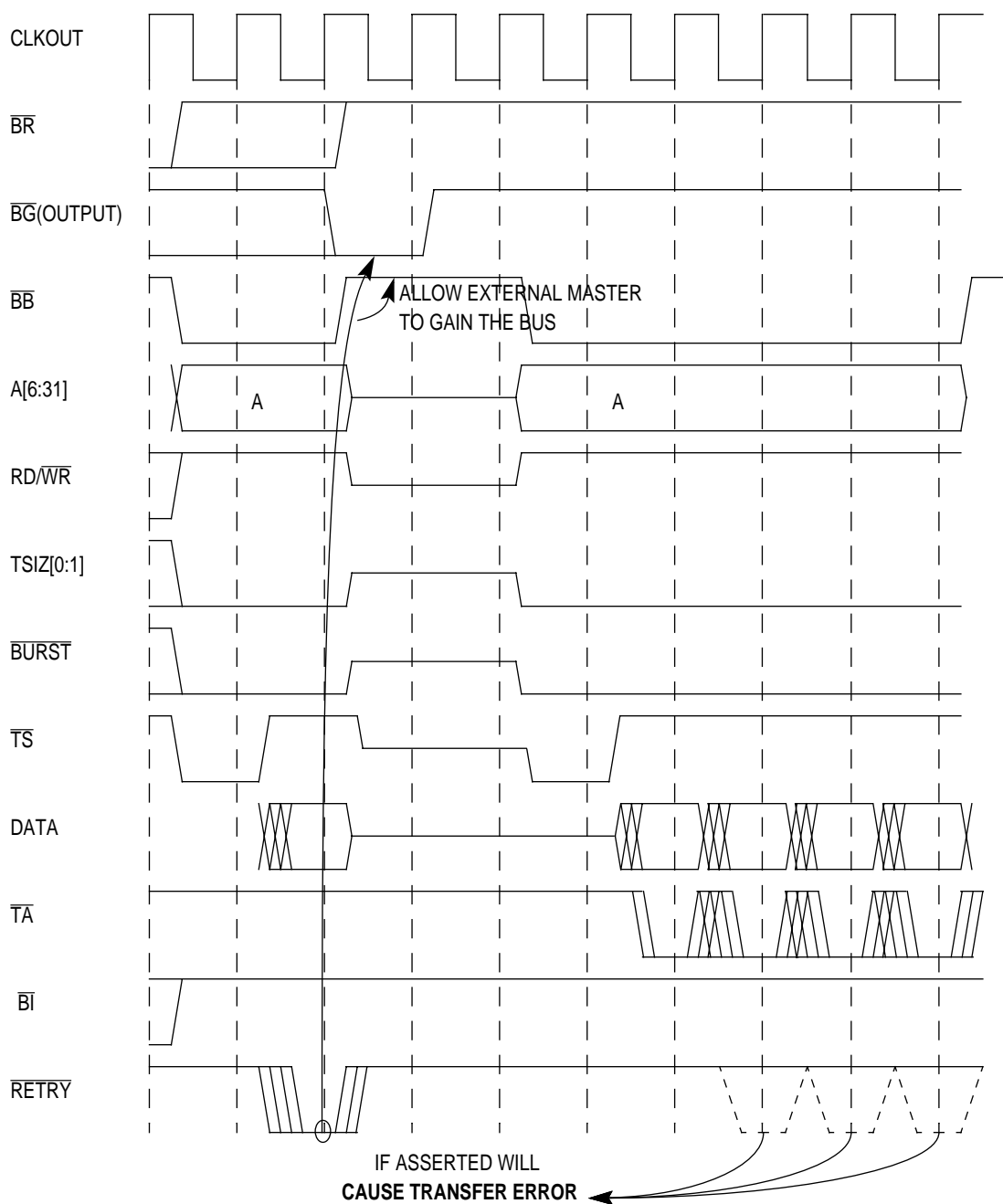
Figure 13-30. Retry On Burst Cycle
