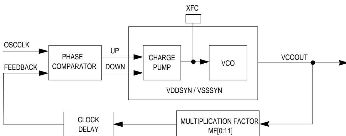
Figure 5-4. SPPLL Block Diagram
