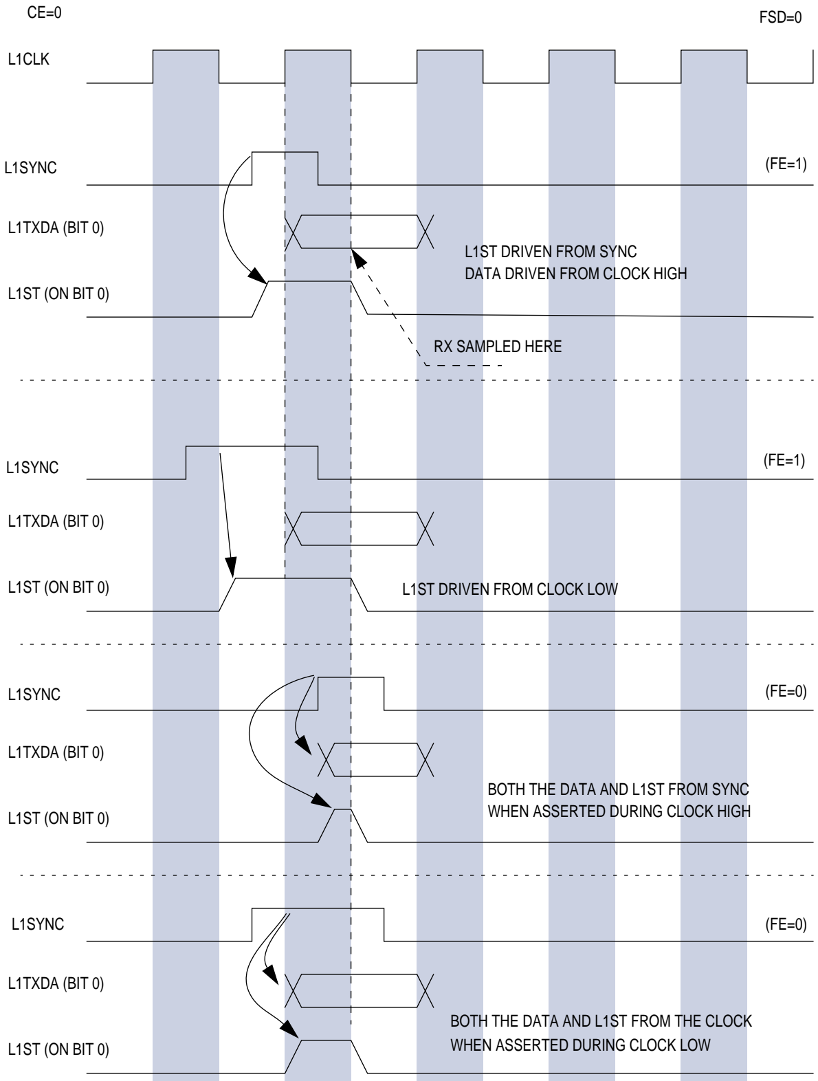
Figure 16-55. Example of CEx = 0 and FEx Interaction, XFSD = 0
