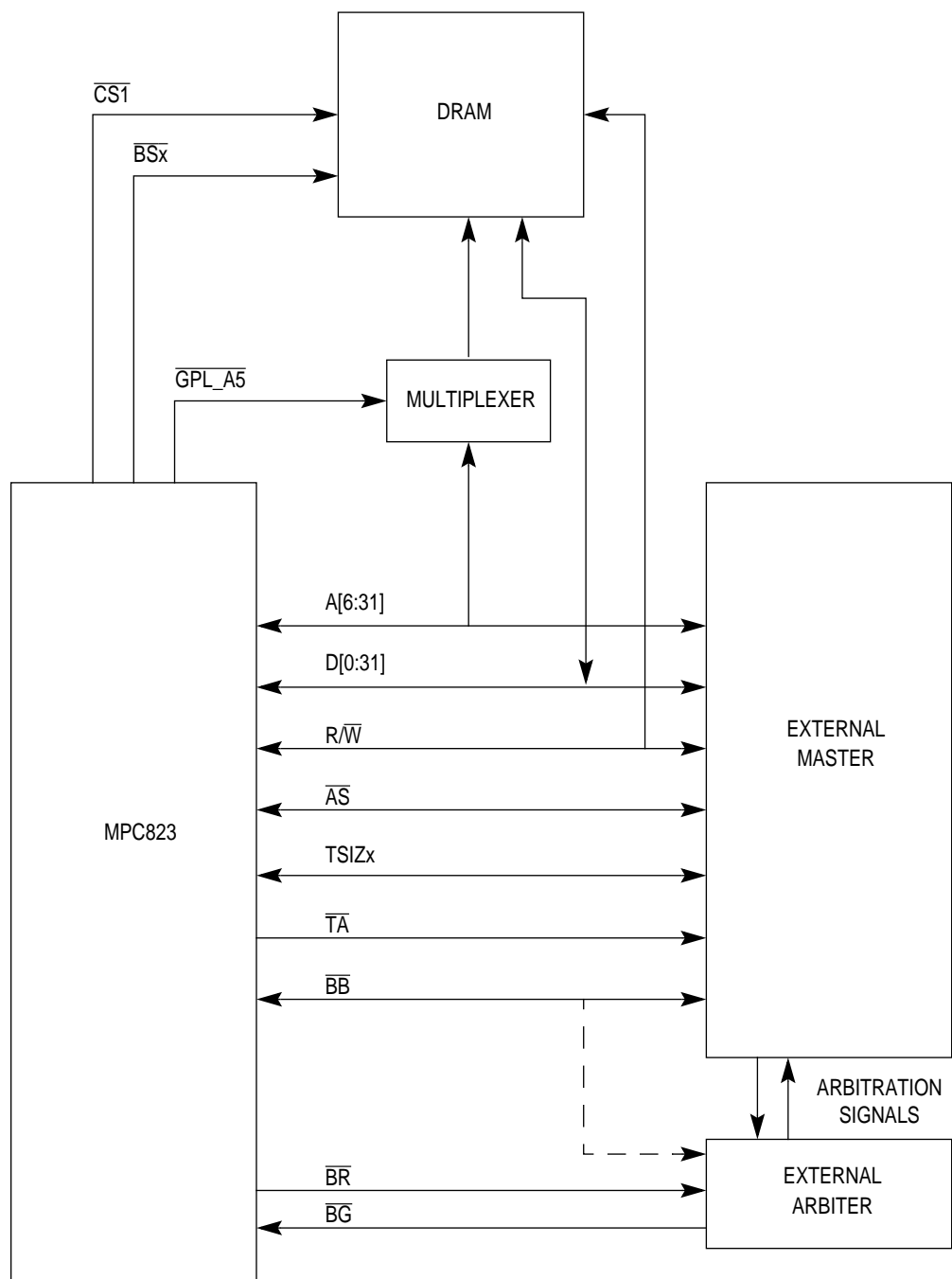
Figure 15-39. Asynchronous External Master Interconnect Example
