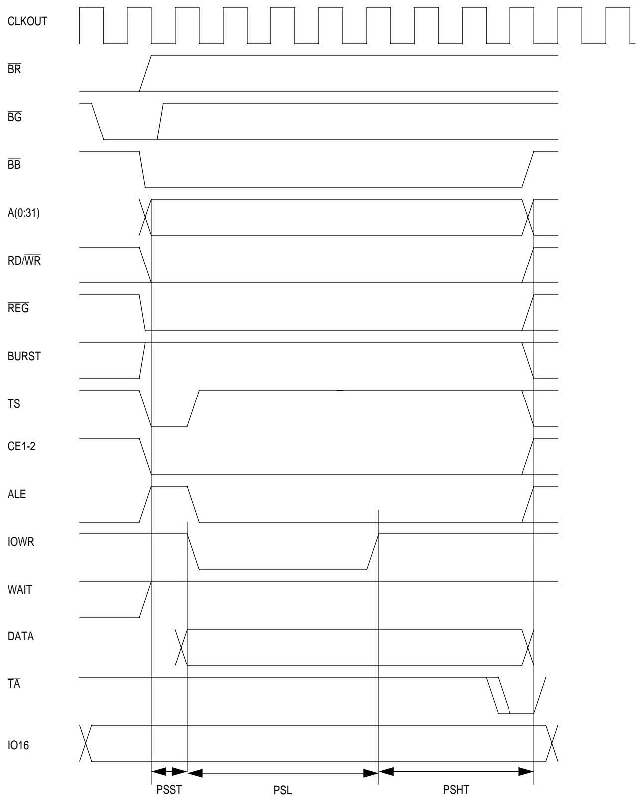
Figure 17-7. PCMCIA Single Beat Write Cycle PRS = 3 PSST = 1 PSL = 4 PSHT = 3
