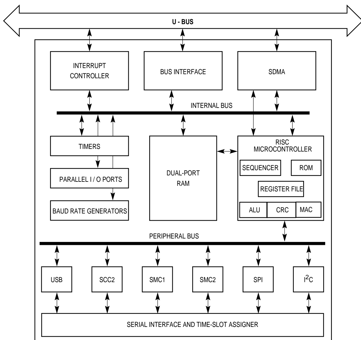
Figure 16-1. CPM Block Diagram
