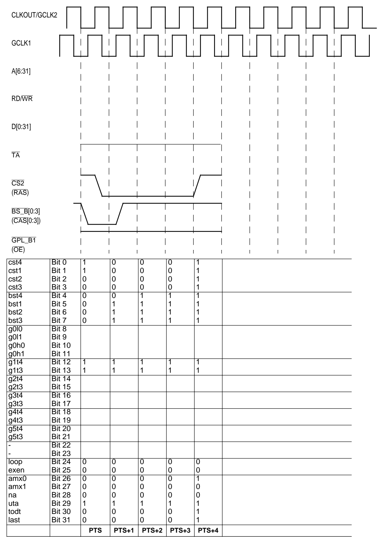
Figure 15-56. EDO DRAM Refresh Cycle (CAS Before RAS)
