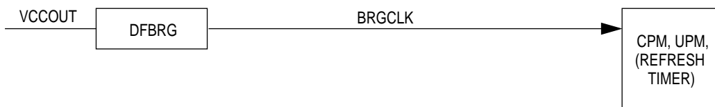
Figure 5-11. BRGCLK Divider
