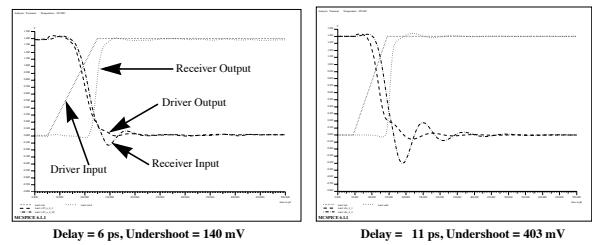
FIGURE 7. Partial (left) vs. Loop inductance model (right) Circuit area: 350 μm * 350 μm
