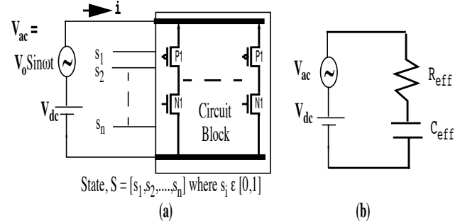
FIGURE 5. Determination of device decoupling cap
