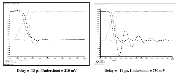
FIGURE 8. Partial (left) vs. Loop inductance model (right) Circuit area: 700 μm * 350 μm
