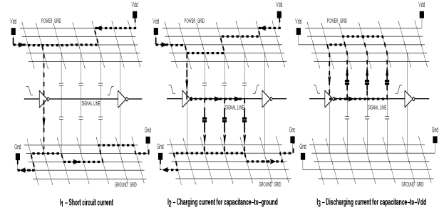
FIGURE 2. Currents in Driver-Receiver-Grid topology
