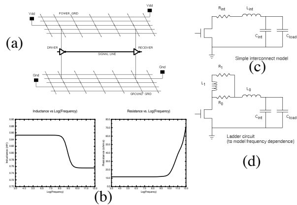
FIGURE 1. Typical grid topology, R & L vs. frequency
